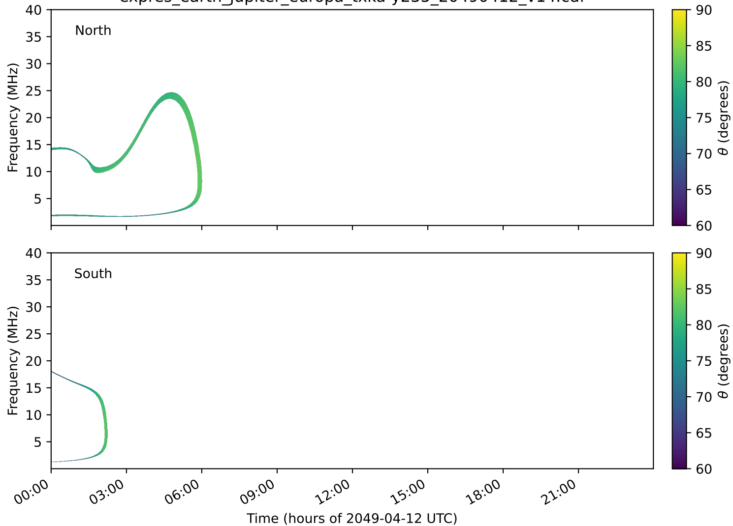
expres_earth_jupiter_europa_txka-y235_20490412_v14.cdf
