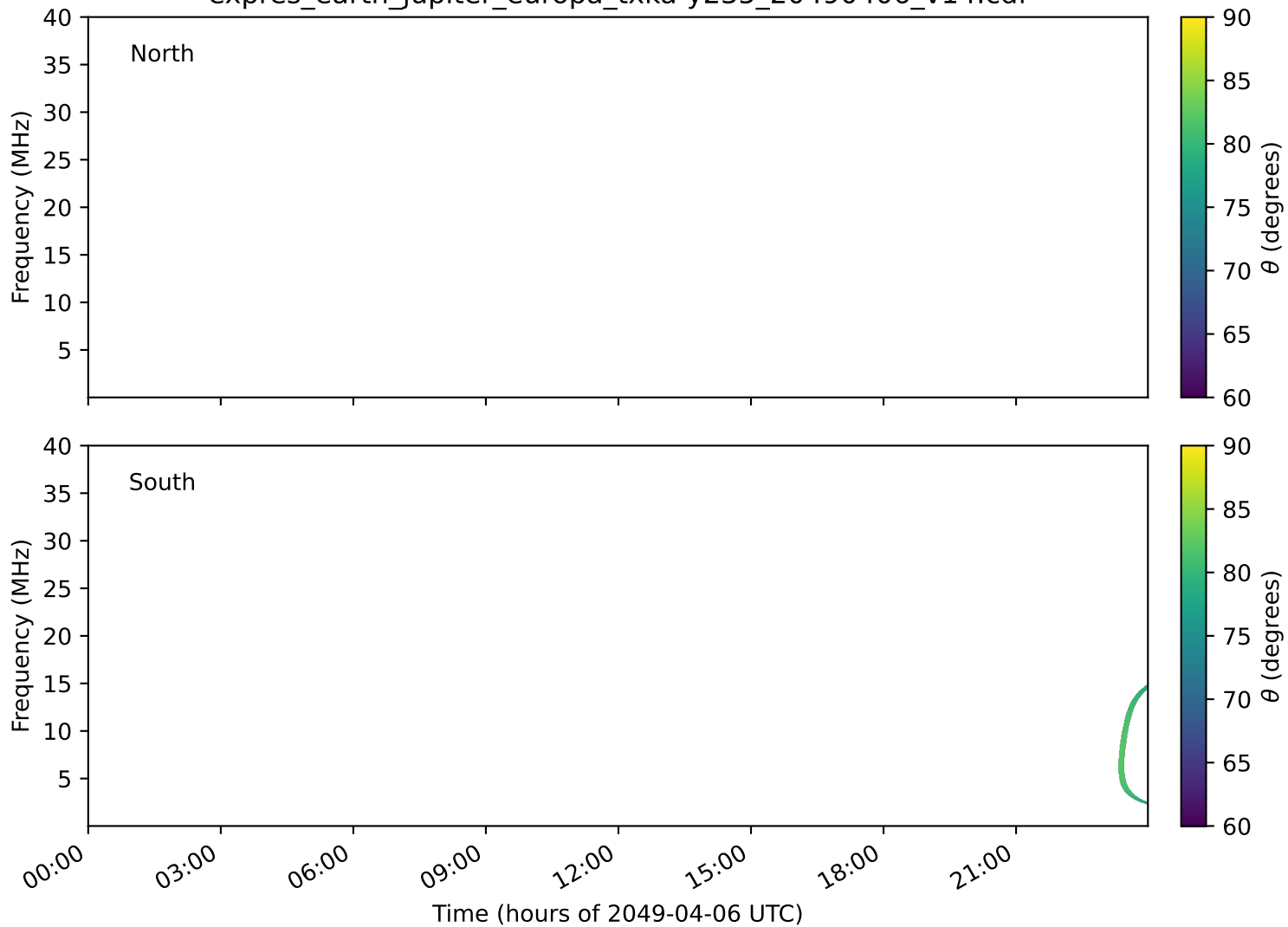
expres_earth_jupiter_europa_txka-y235_20490406_v14.cdf
