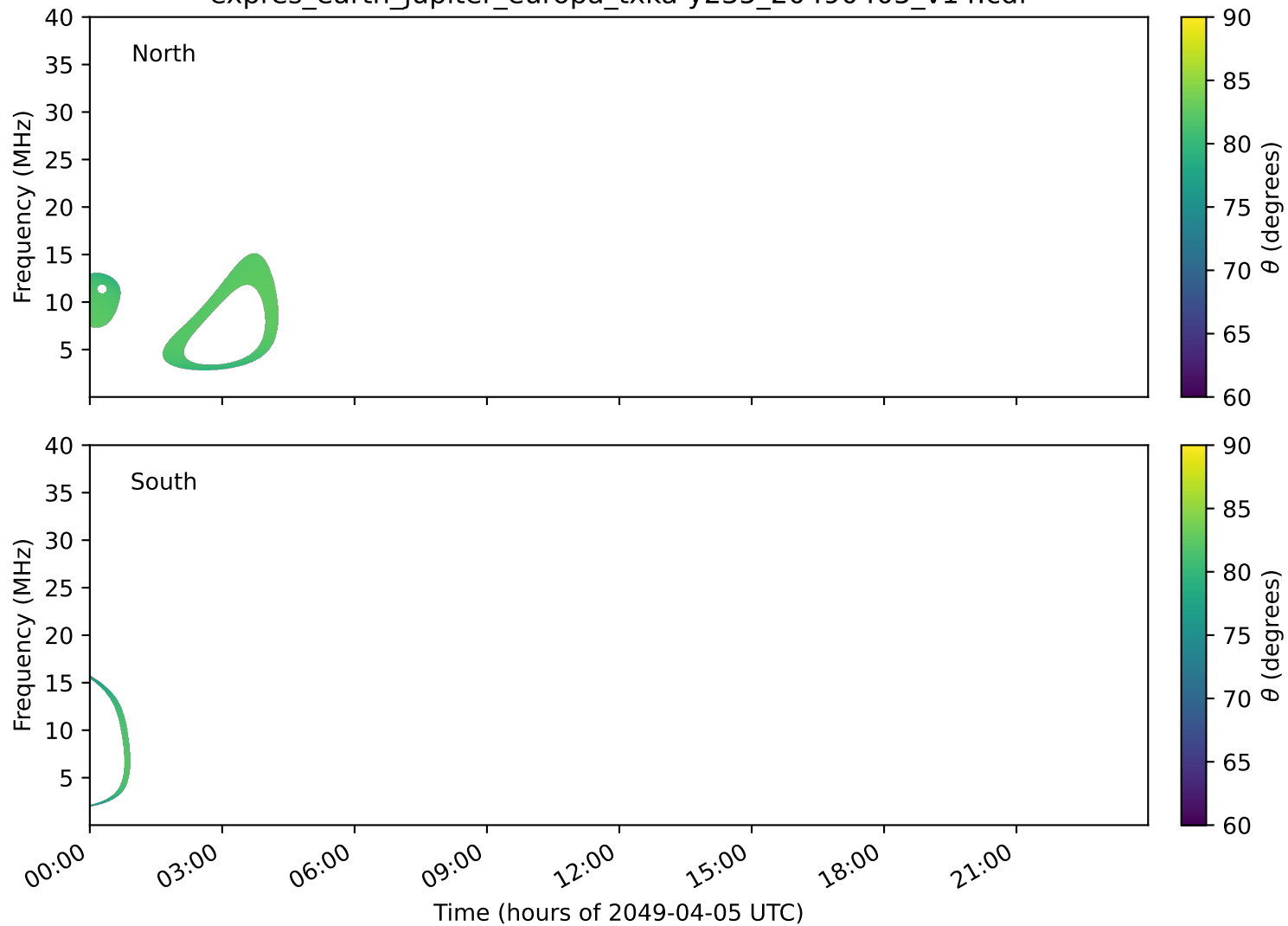
expres_earth_jupiter_europa_txka-y235_20490405_v14.cdf
