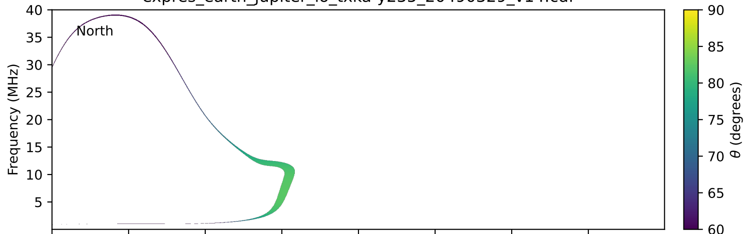
expres_earth_jupiter_io_txka-y235_20490329_v14.cdf
