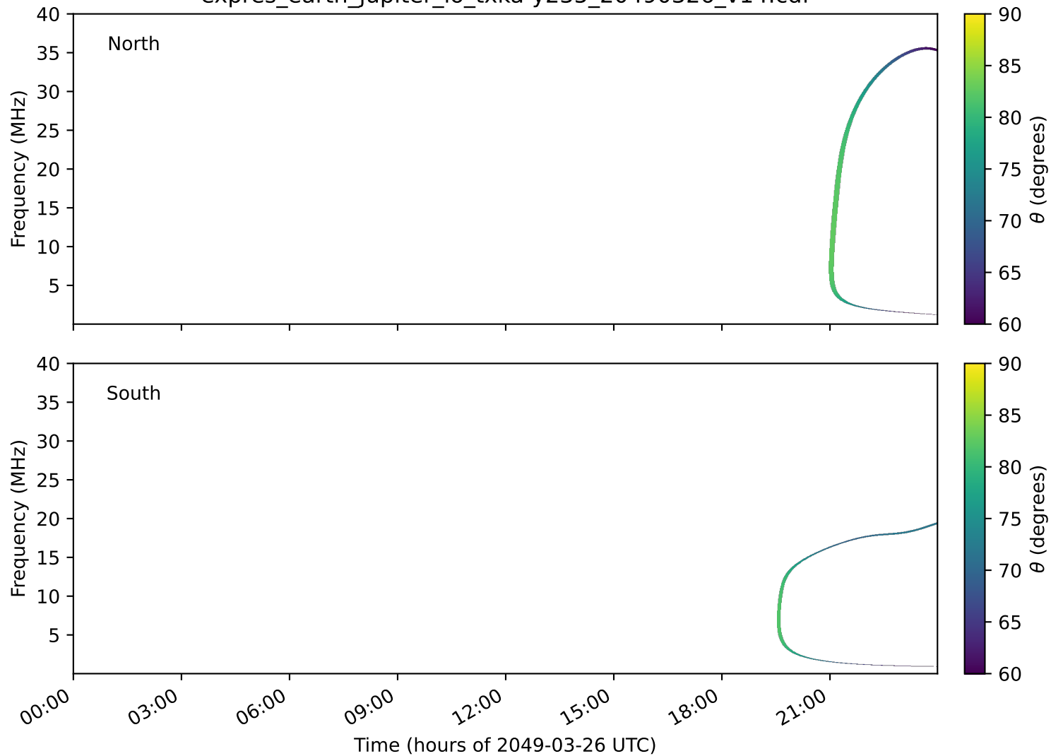
expres_earth_jupiter_io_txka-y235_20490326_v14.cdf
