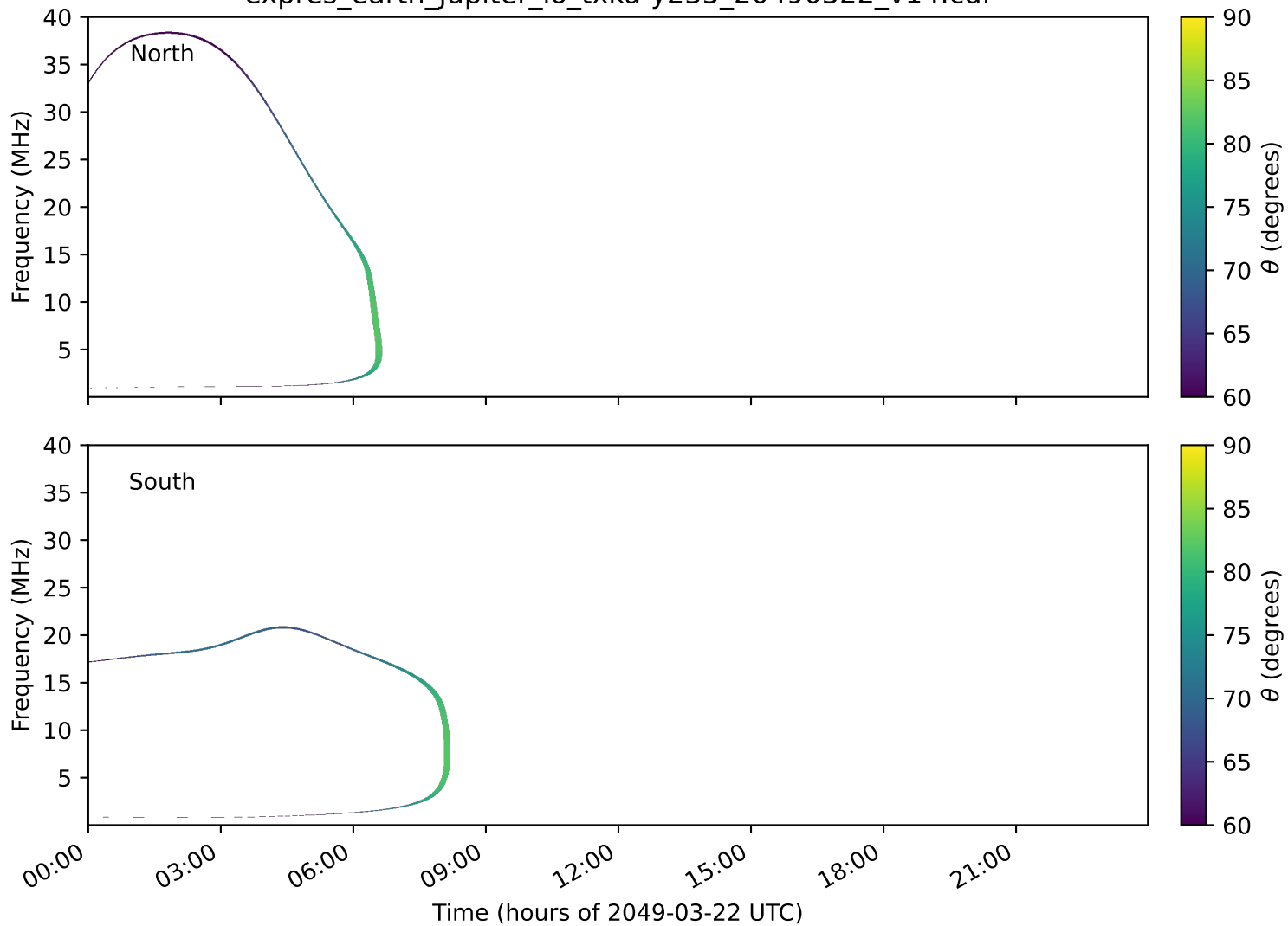
expres_earth_jupiter_io_txka-y235_20490322_v14.cdf
