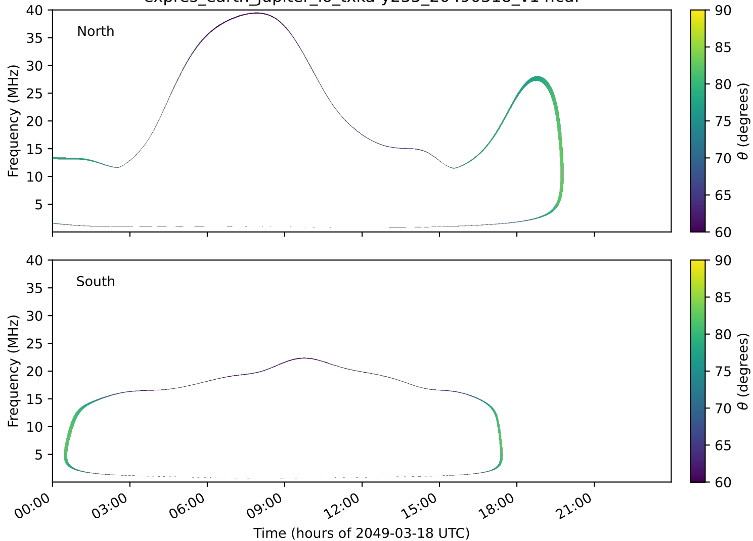
expres_earth_jupiter_io_txka-y235_20490318_v14.cdf
