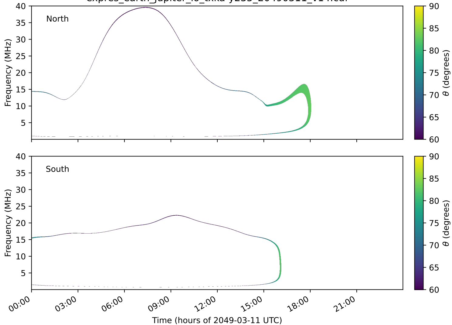
expres_earth_jupiter_io_txka-y235_20490311_v14.cdf
