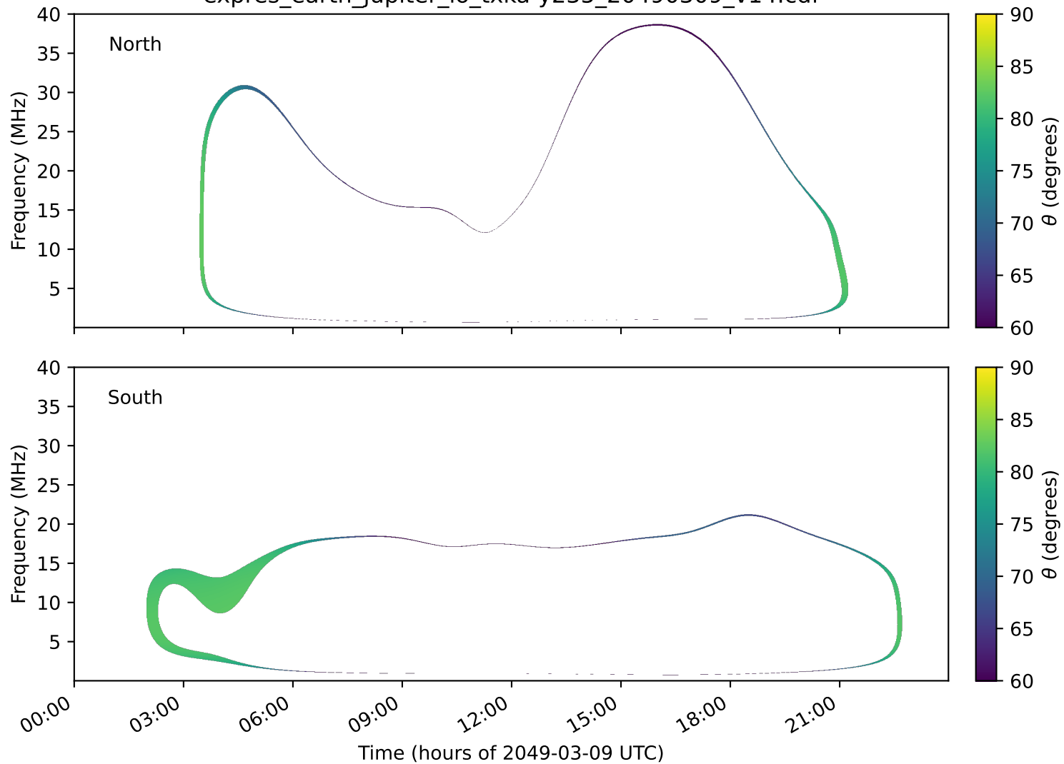
expres_earth_jupiter_io_txka-y235_20490309_v14.cdf
