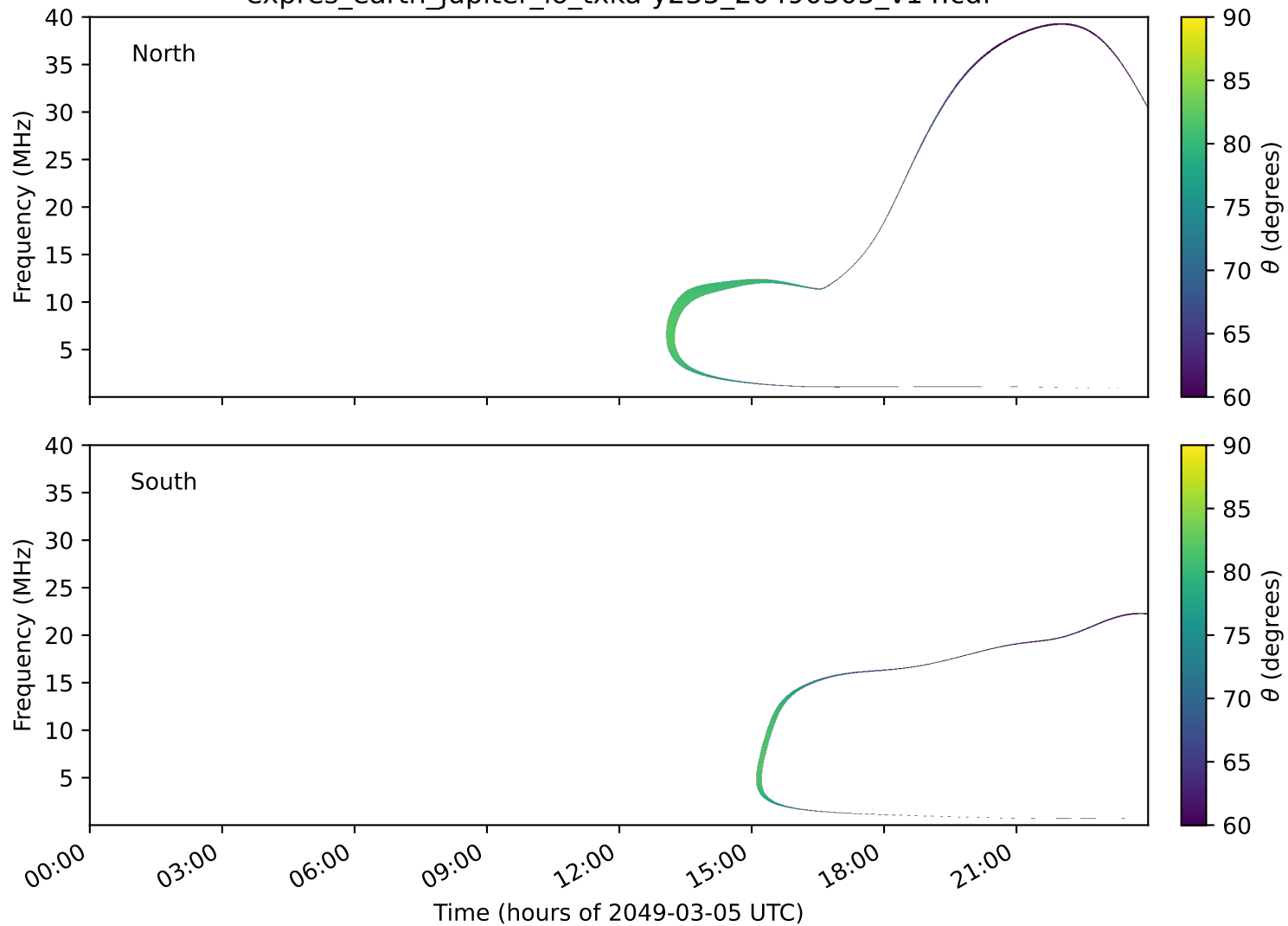
expres_earth_jupiter_io_txka-y235_20490305_v14.cdf
