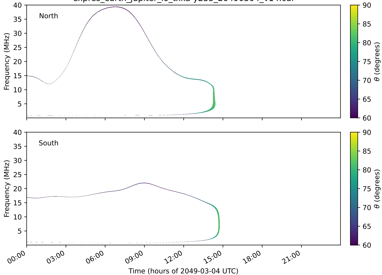
expres_earth_jupiter_io_txka-y235_20490304_v14.cdf
