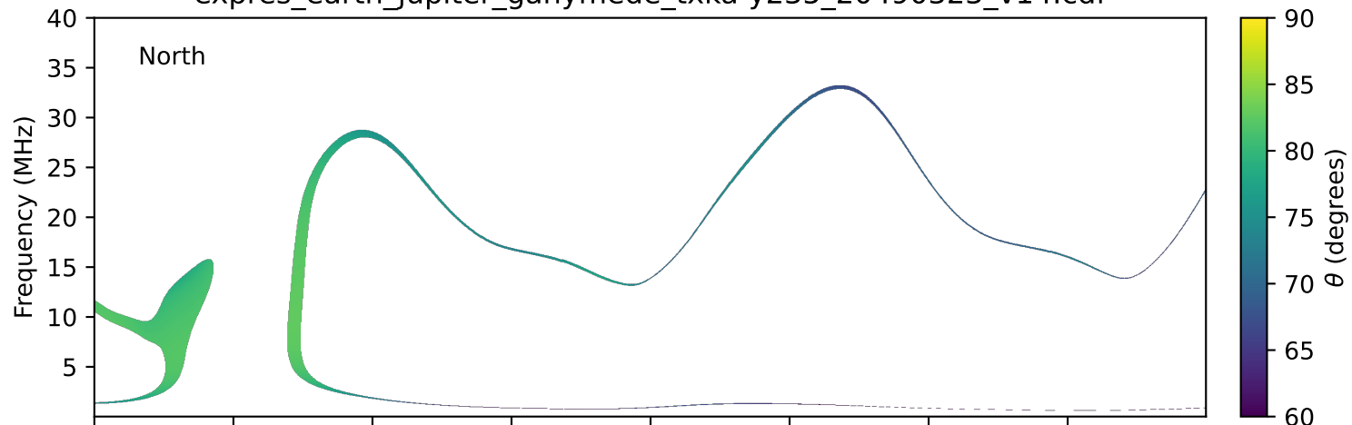
expres_earth_jupiter_ganymede_txka-y235_20490323_v14.cdf
