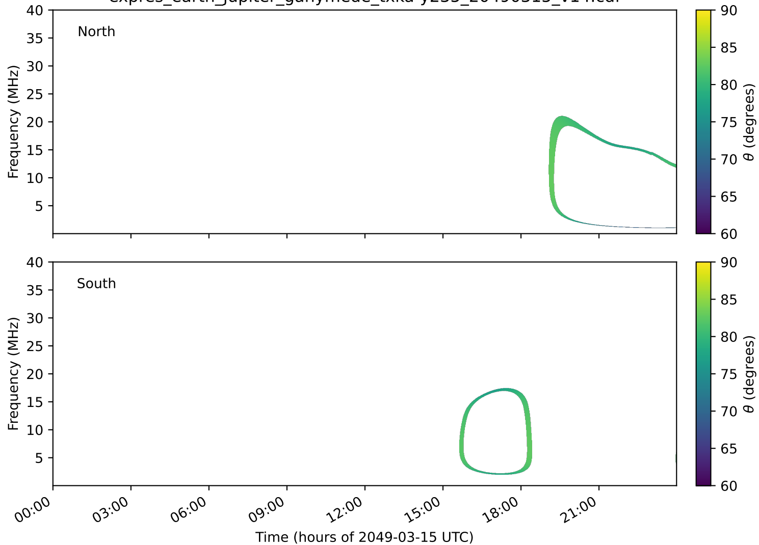
expres_earth_jupiter_ganymede_txka-y235_20490315_v14.cdf
