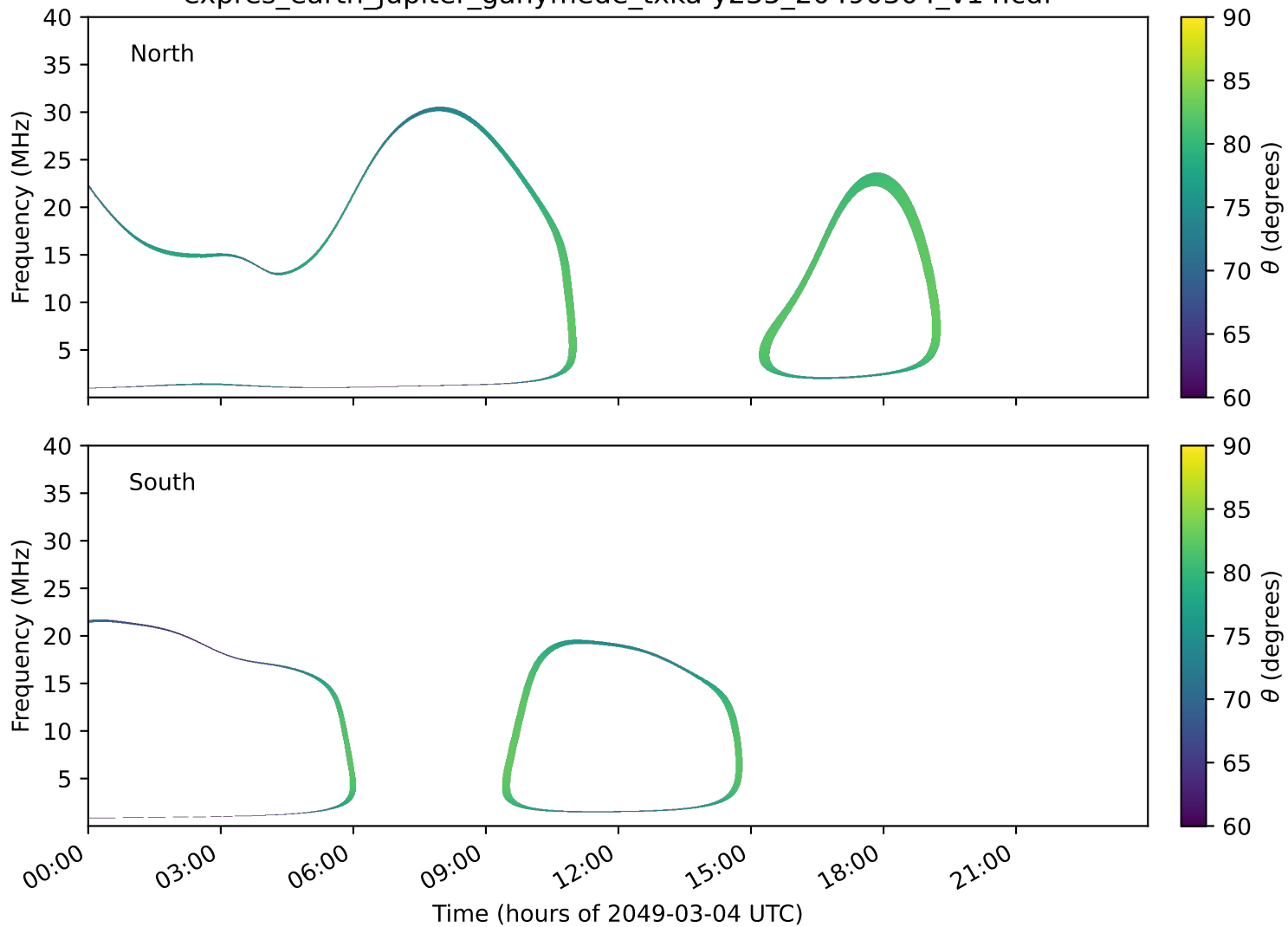
expres_earth_jupiter_ganymede_txka-y235_20490304_v14.cdf
