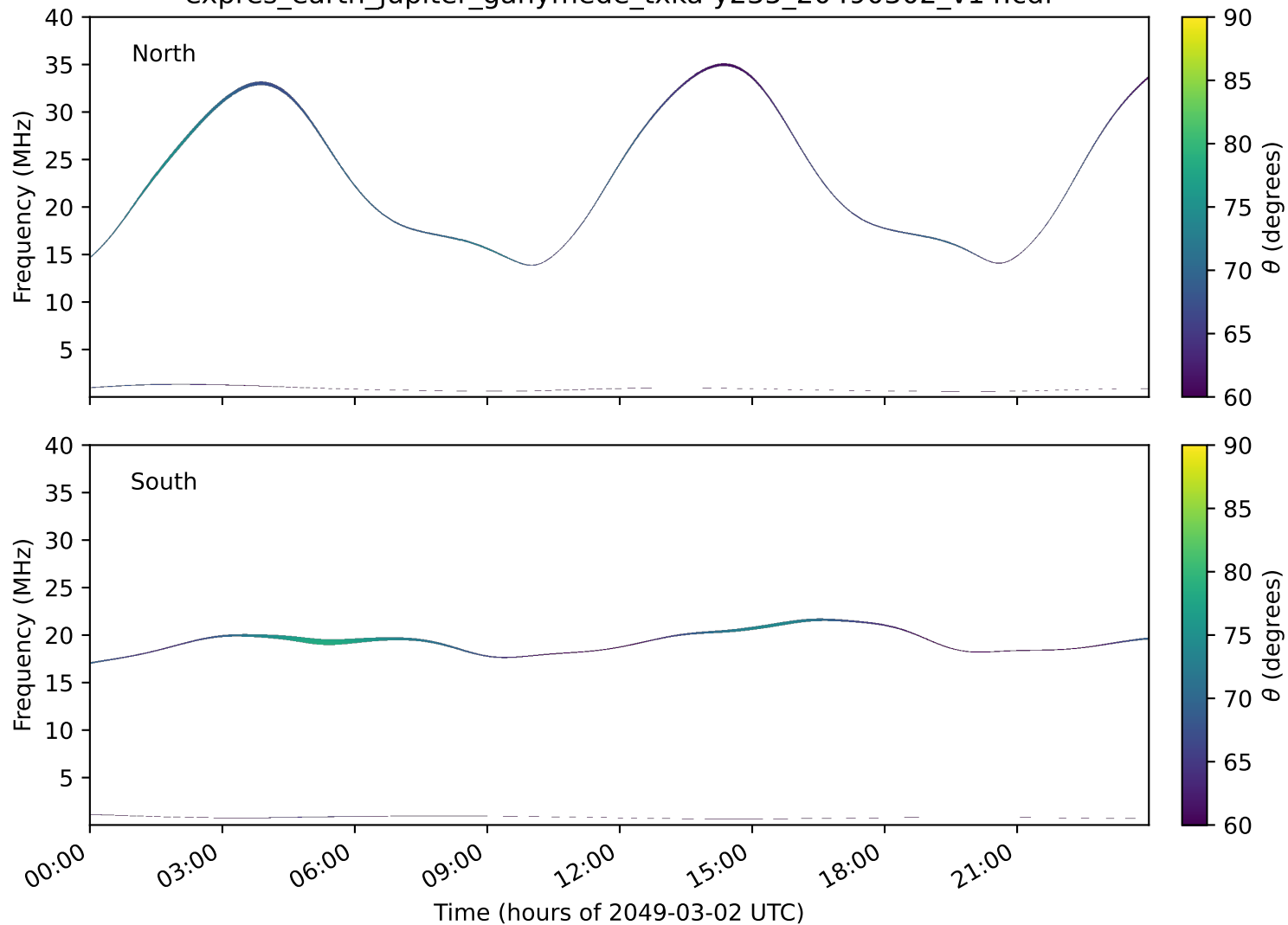
expres_earth_jupiter_ganymede_txka-y235_20490302_v14.cdf
