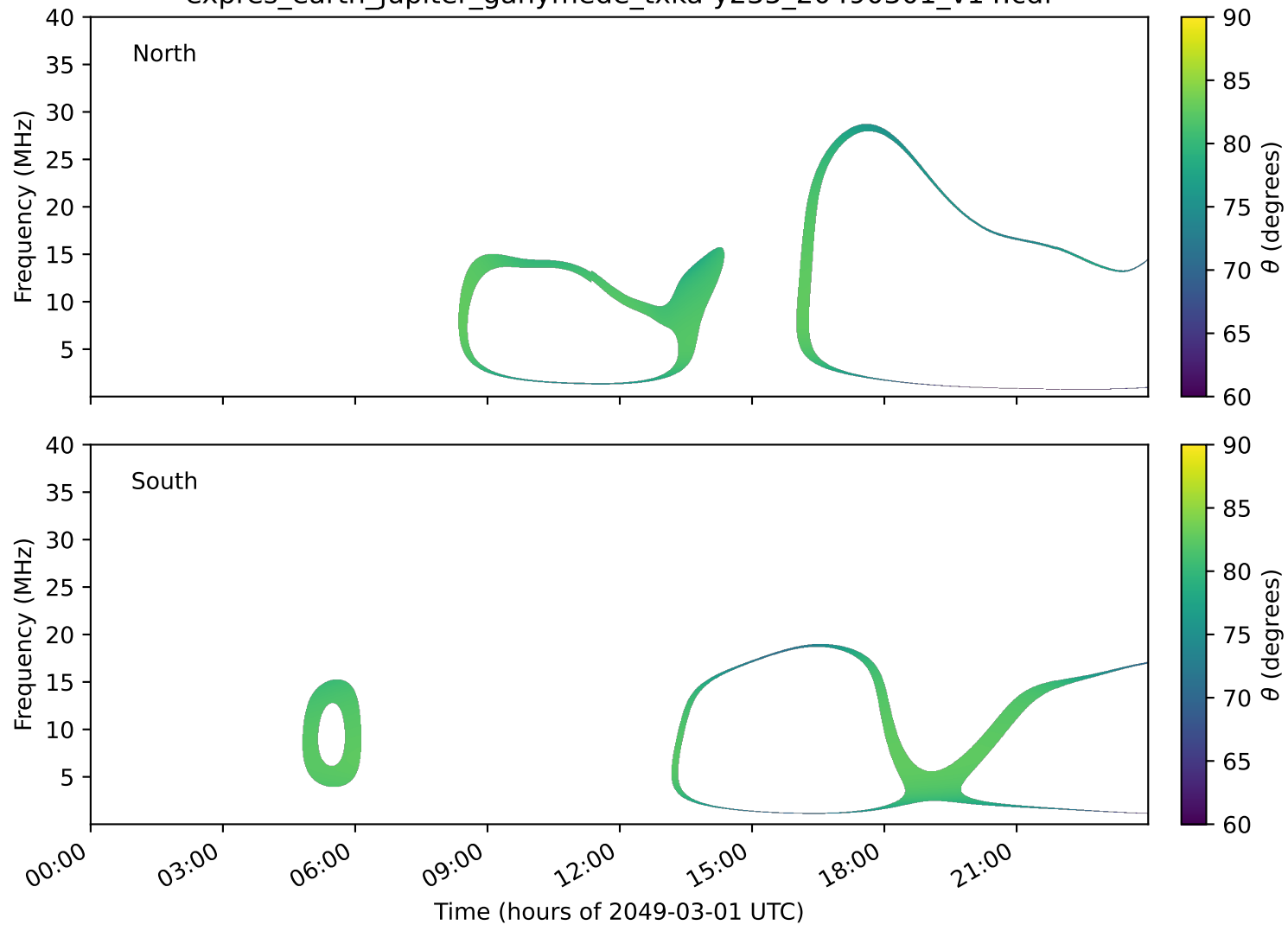
expres_earth_jupiter_ganymede_txka-y235_20490301_v14.cdf
