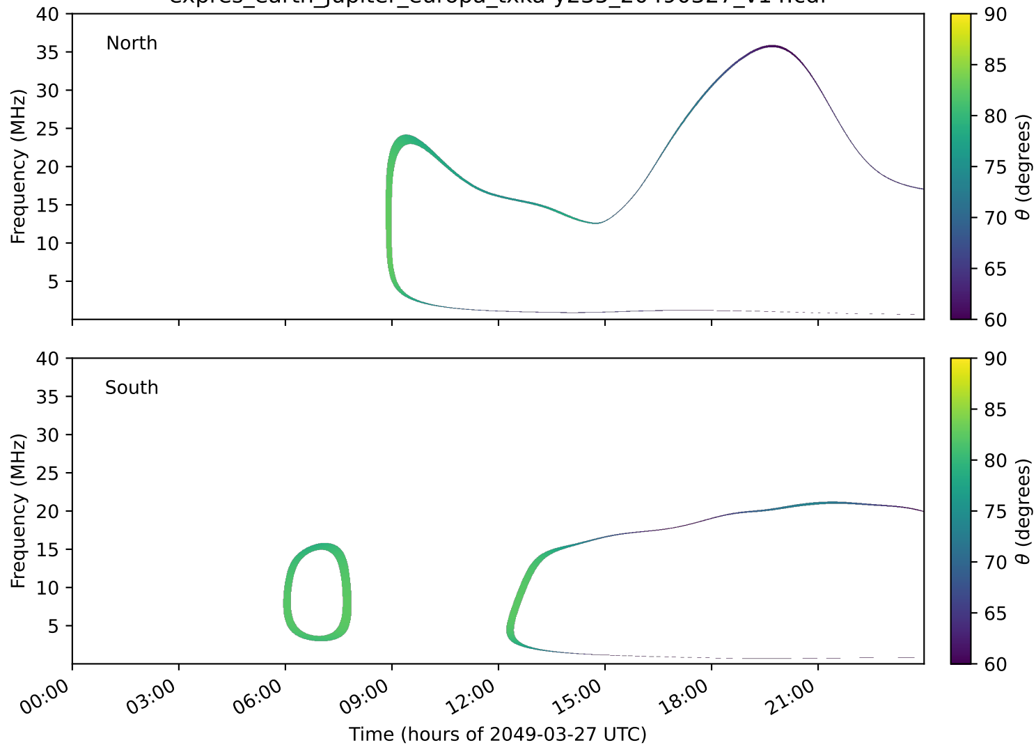
expres_earth_jupiter_europa_txka-y235_20490327_v14.cdf
