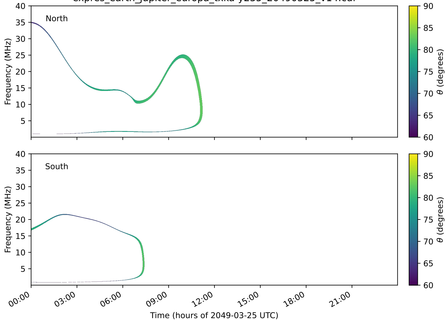
expres_earth_jupiter_europa_txka-y235_20490325_v14.cdf
