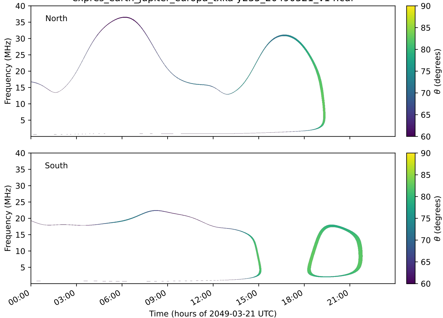
expres_earth_jupiter_europa_txka-y235_20490321_v14.cdf
