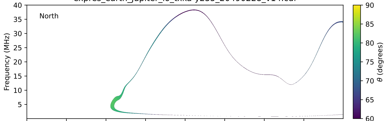
expres_earth_jupiter_io_txka-y235_20490228_v14.cdf
