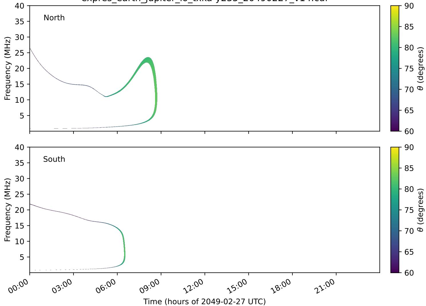
expres_earth_jupiter_io_txka-y235_20490227_v14.cdf
