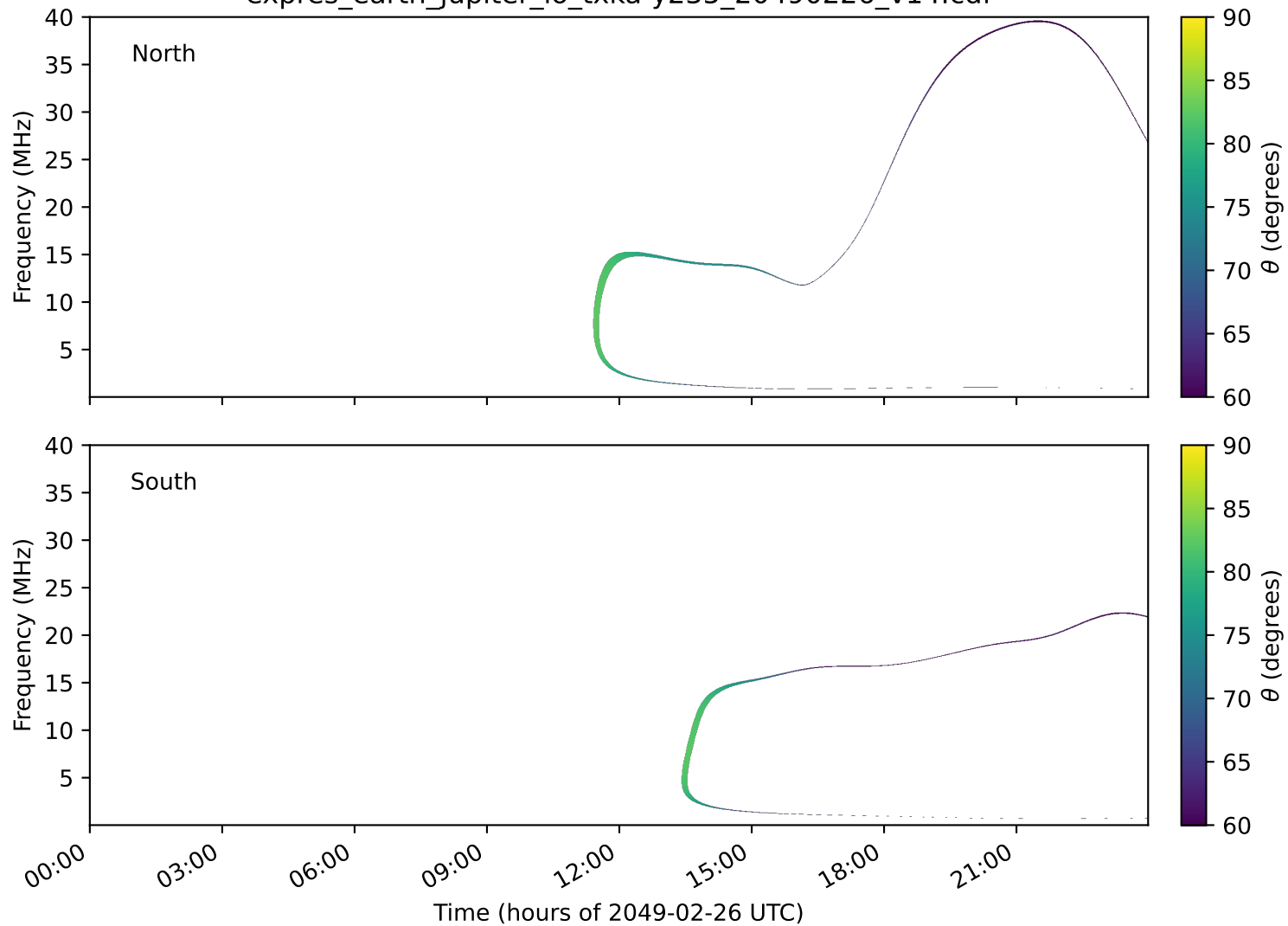
expres_earth_jupiter_io_txka-y235_20490226_v14.cdf
