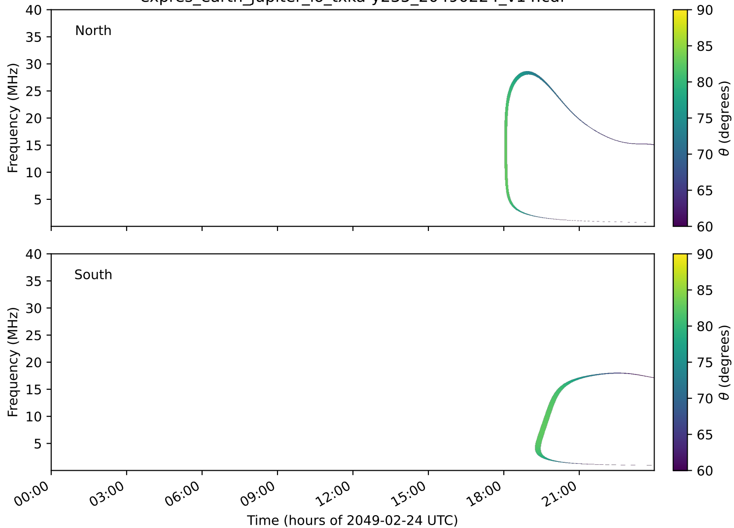
expres_earth_jupiter_io_txka-y235_20490224_v14.cdf
