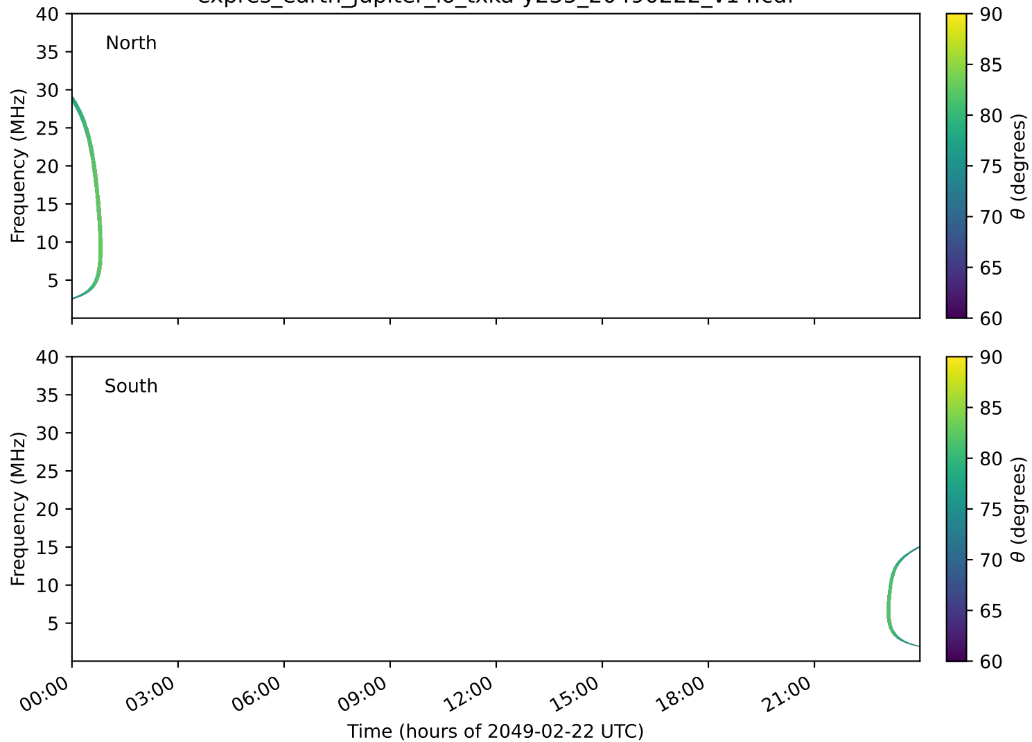
expres_earth_jupiter_io_txka-y235_20490222_v14.cdf
