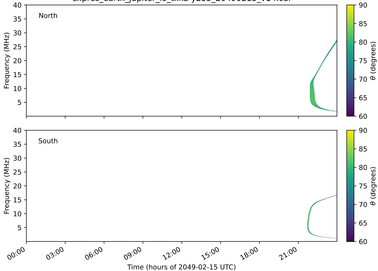
expres_earth_jupiter_io_txka-y235_20490215_v14.cdf
