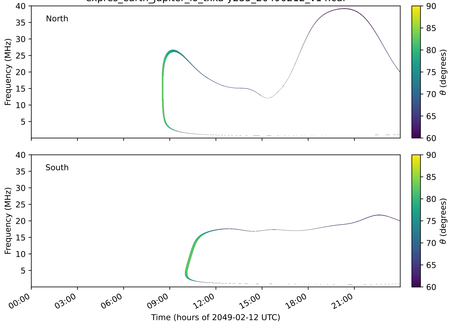
expres_earth_jupiter_io_txka-y235_20490212_v14.cdf
