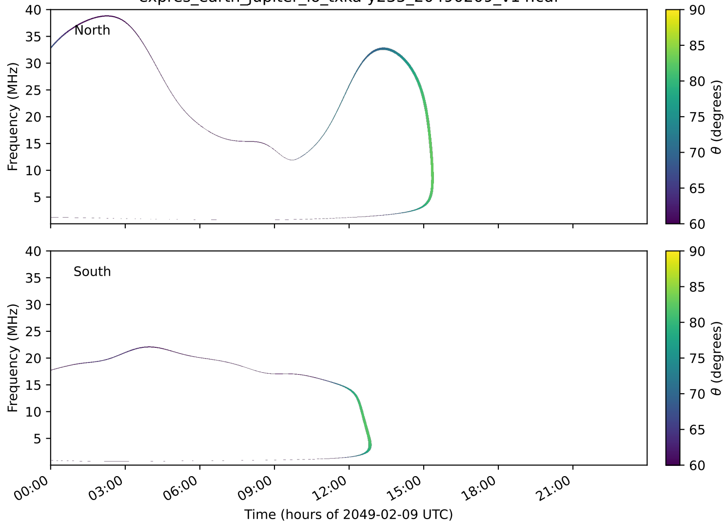
expres_earth_jupiter_io_txka-y235_20490209_v14.cdf
