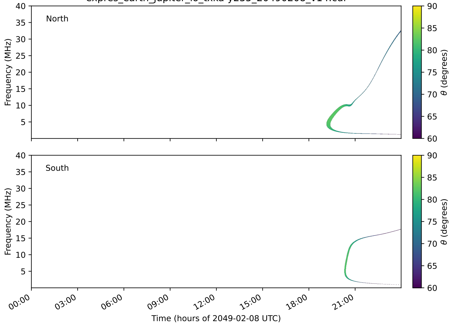
expres_earth_jupiter_io_txka-y235_20490208_v14.cdf
