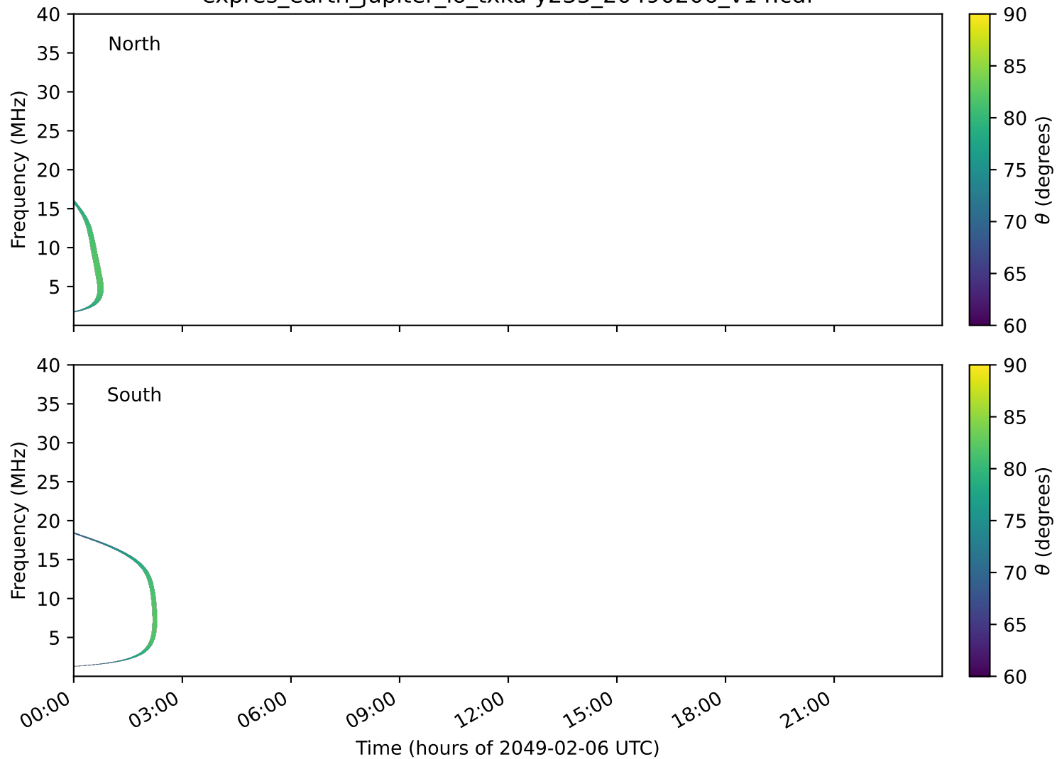
expres_earth_jupiter_io_txka-y235_20490206_v14.cdf
