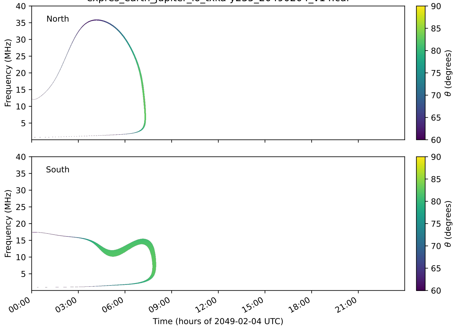
expres_earth_jupiter_io_txka-y235_20490204_v14.cdf
