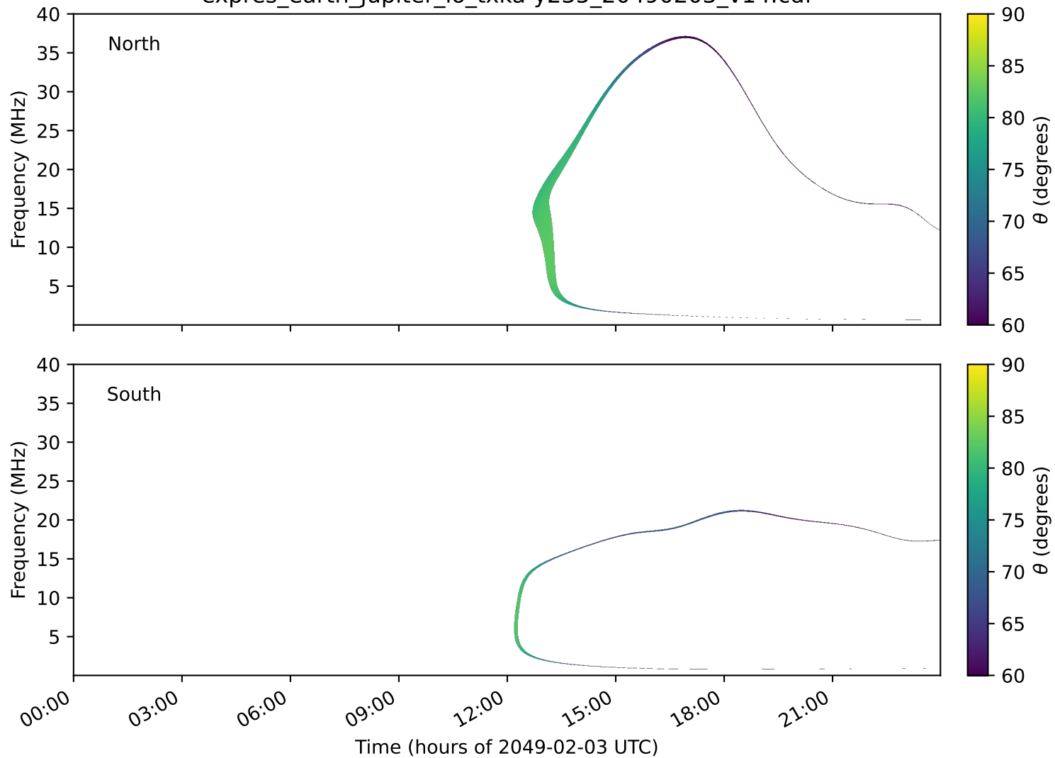
expres_earth_jupiter_io_txka-y235_20490203_v14.cdf
