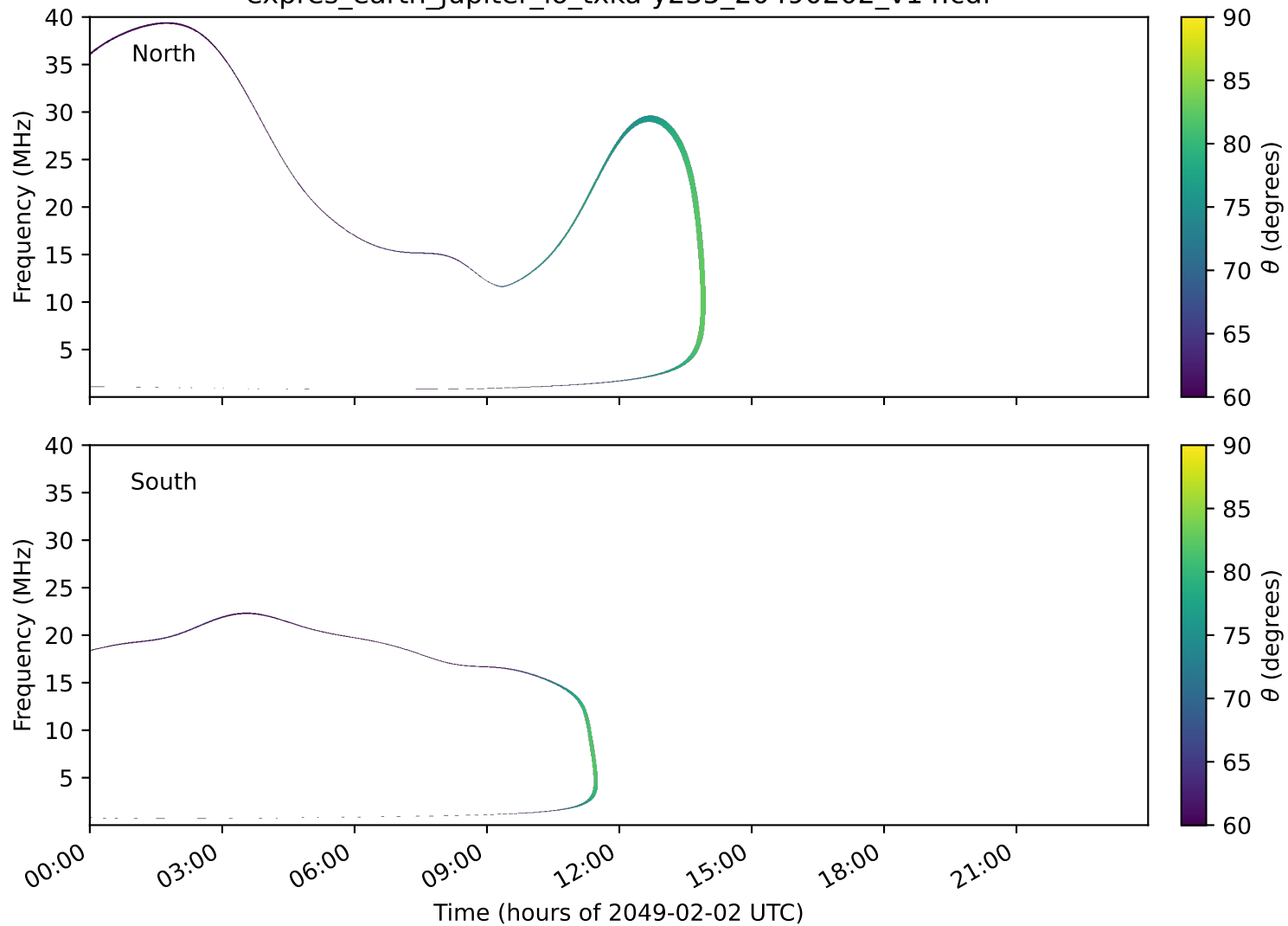
expres_earth_jupiter_io_txka-y235_20490202_v14.cdf
