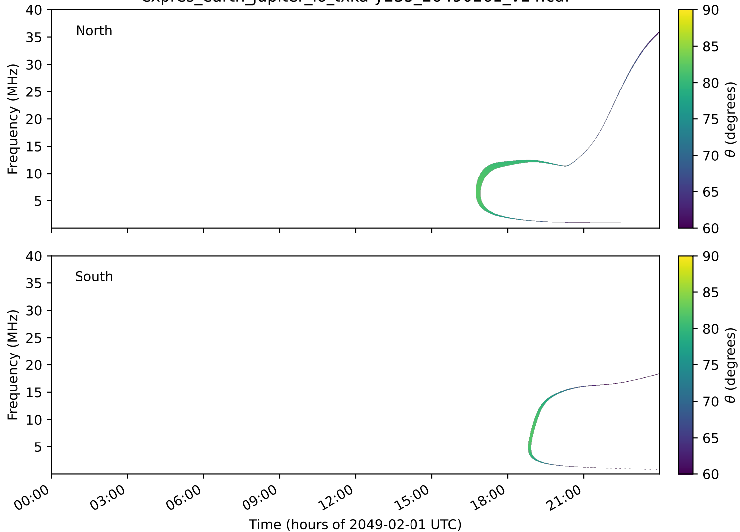
expres_earth_jupiter_io_txka-y235_20490201_v14.cdf
