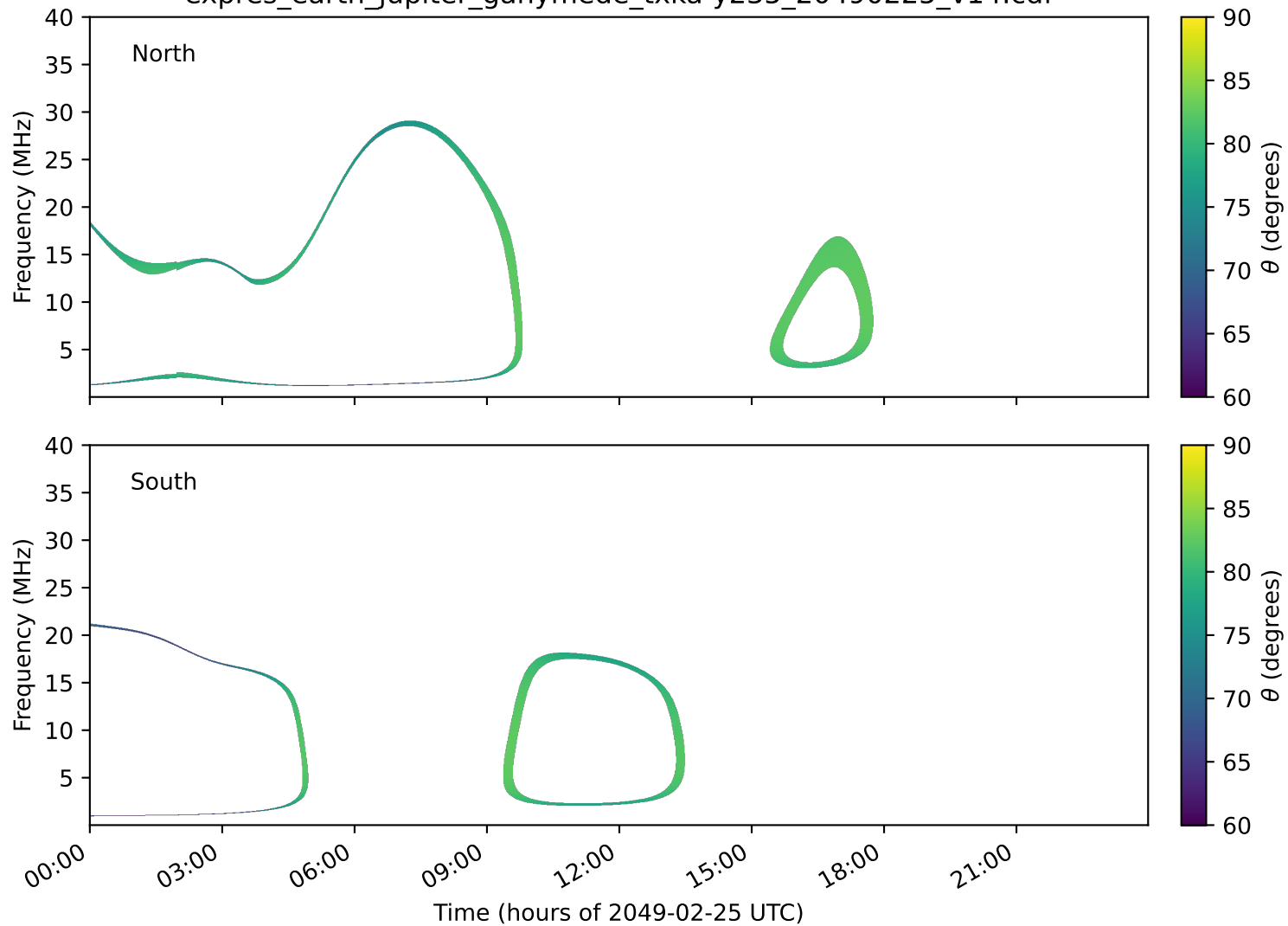
expres_earth_jupiter_ganymede_txka-y235_20490225_v14.cdf
