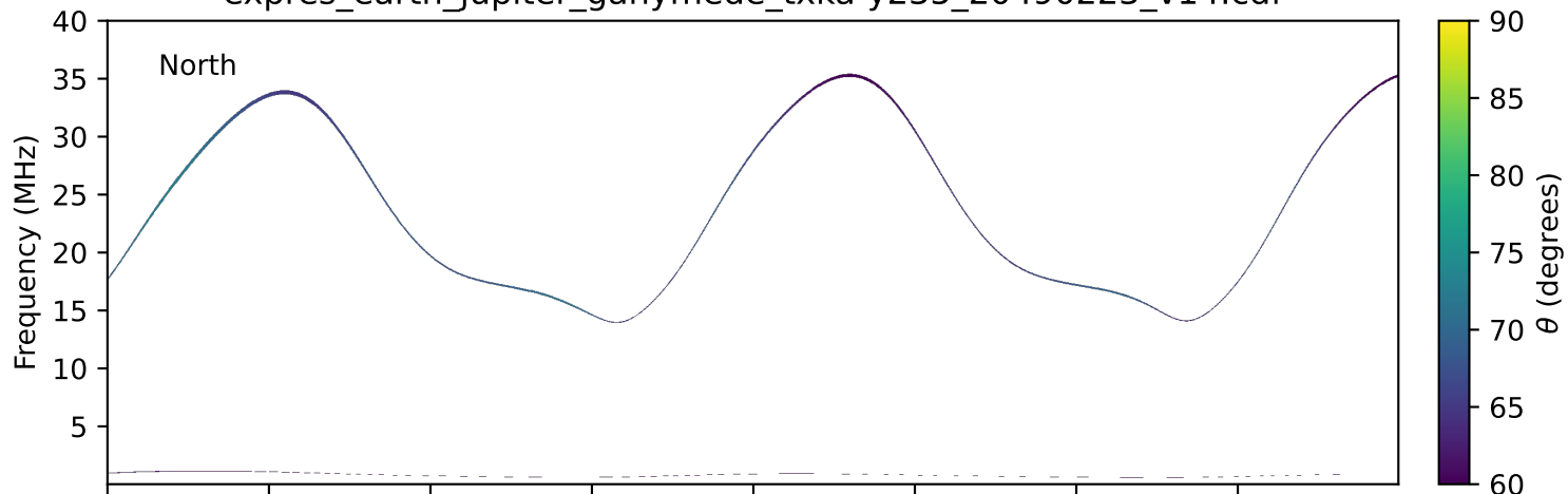
expres_earth_jupiter_ganymede_txka-y235_20490223_v14.cdf
