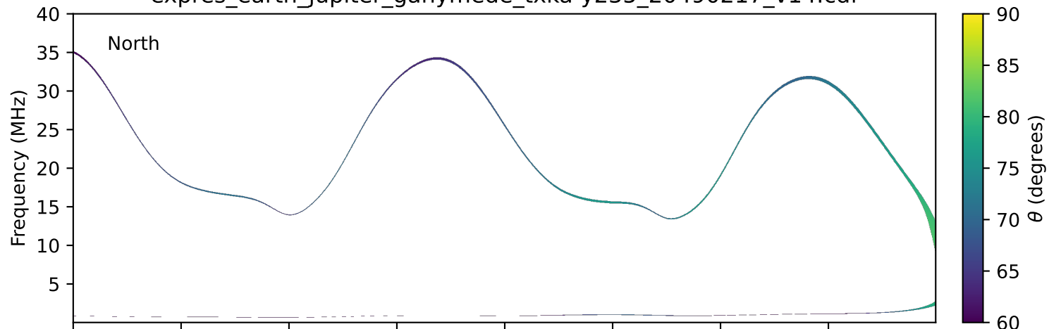
expres_earth_jupiter_ganymede_txka-y235_20490217_v14.cdf
