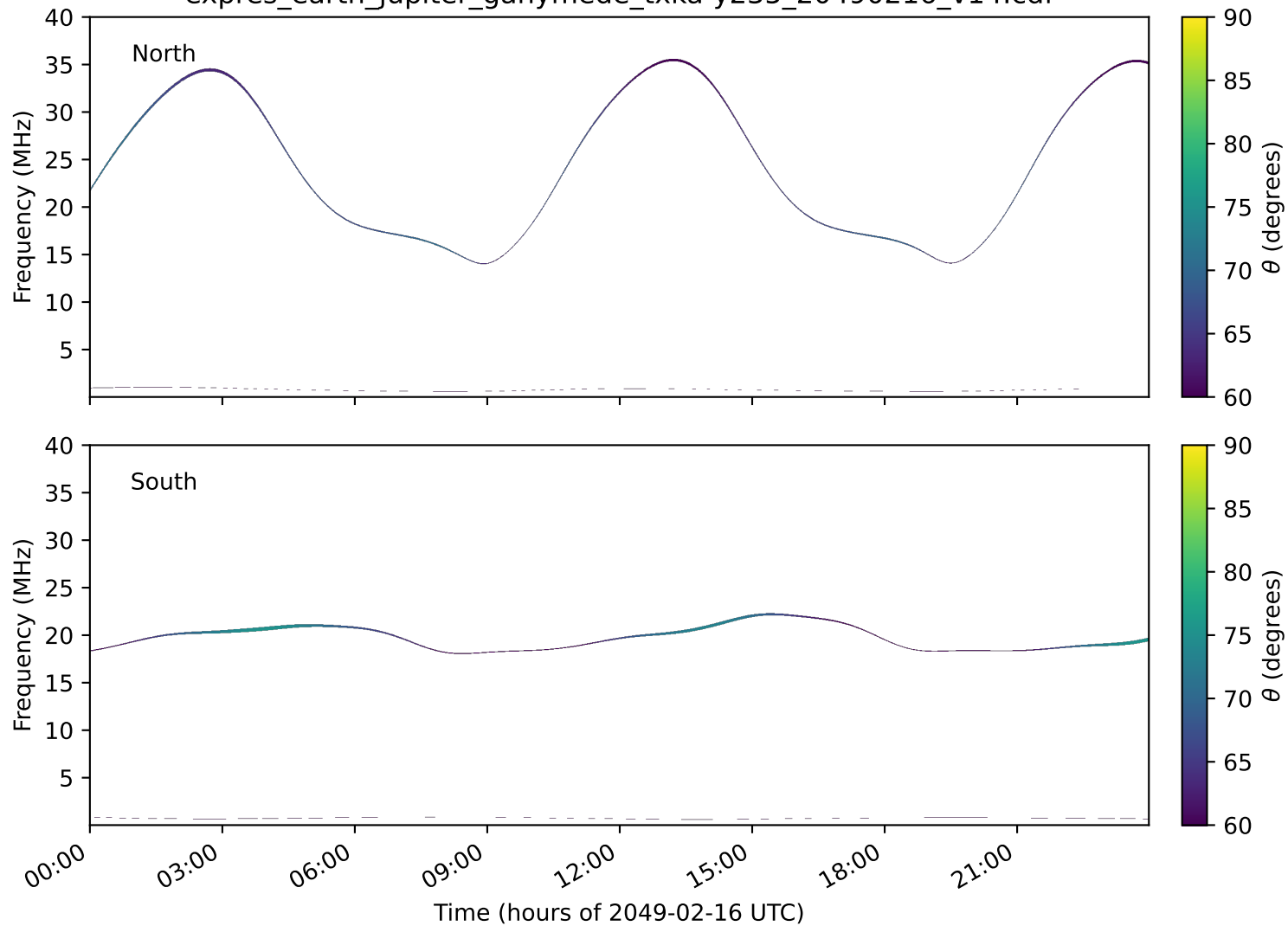
expres_earth_jupiter_ganymede_txka-y235_20490216_v14.cdf
