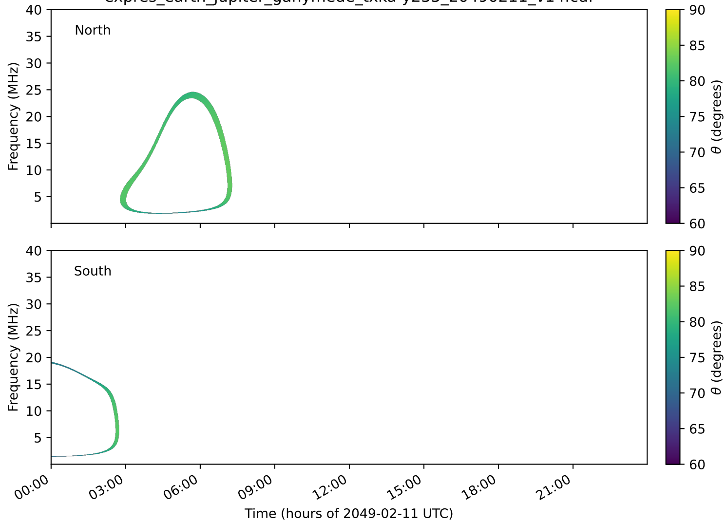
expres_earth_jupiter_ganymede_txka-y235_20490211_v14.cdf
