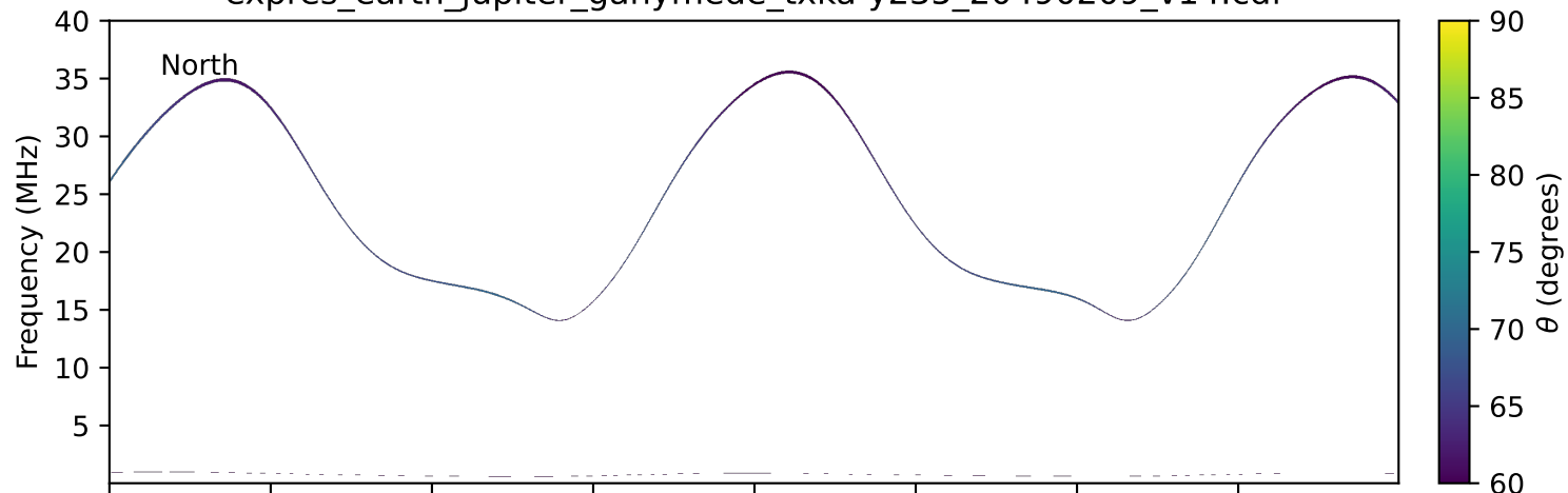
expres_earth_jupiter_ganymede_txka-y235_20490209_v14.cdf
