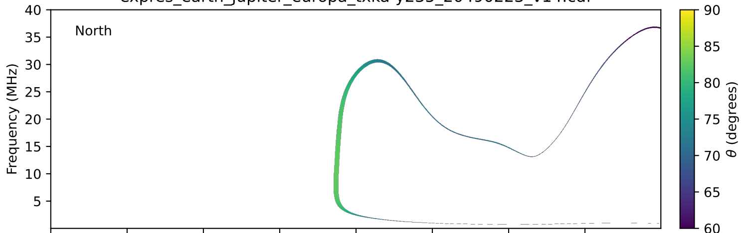
expres_earth_jupiter_europa_txka-y235_20490223_v14.cdf
