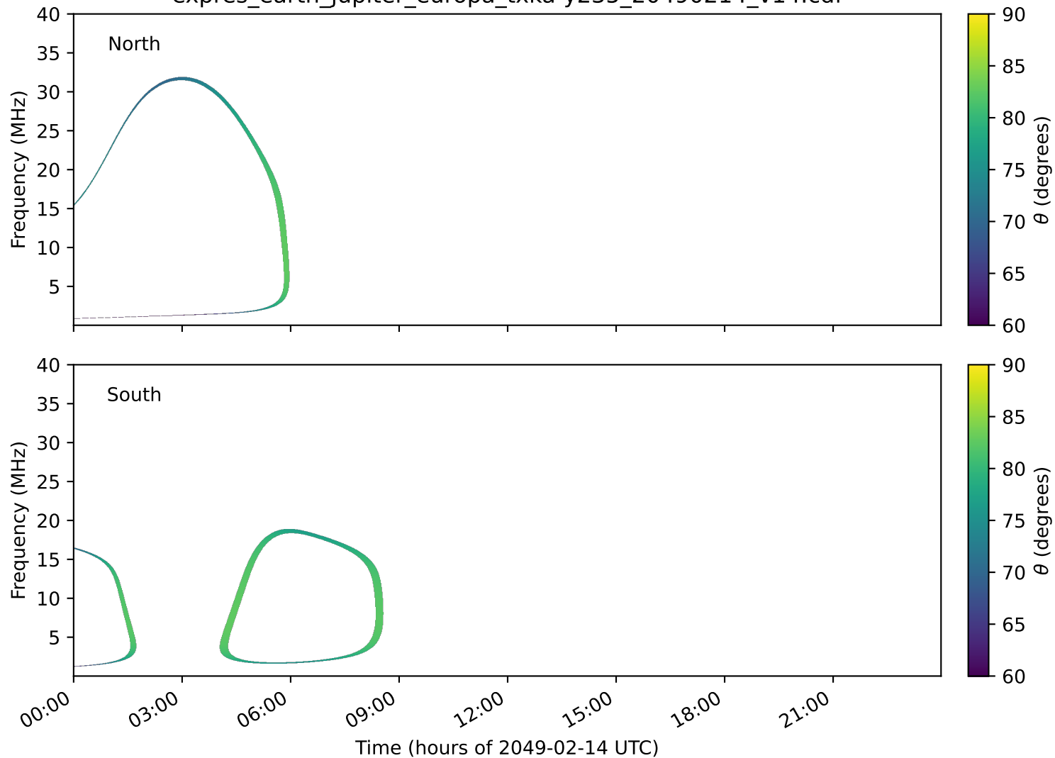
expres_earth_jupiter_europa_txka-y235_20490214_v14.cdf
