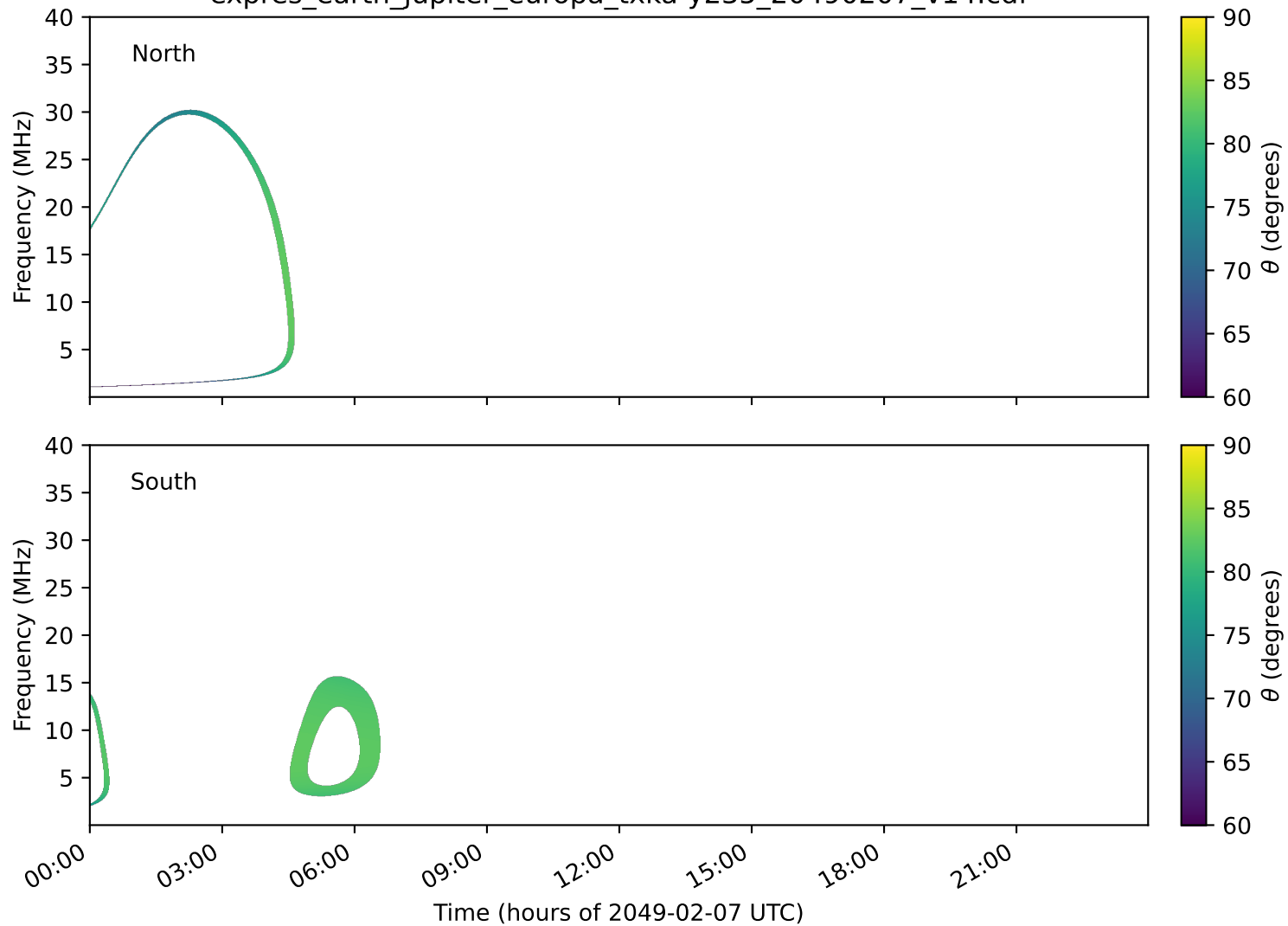
expres_earth_jupiter_europa_txka-y235_20490207_v14.cdf
