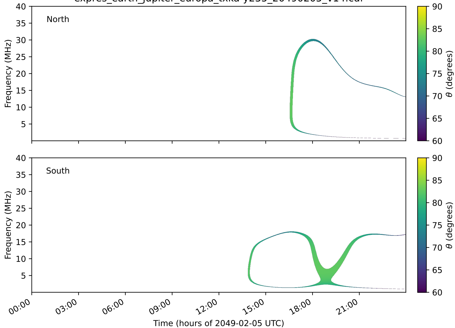
expres_earth_jupiter_europa_txka-y235_20490205_v14.cdf
