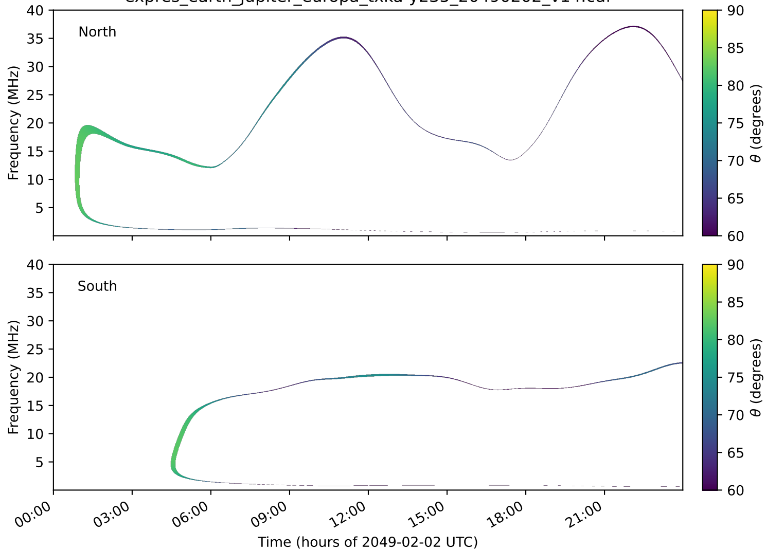
expres_earth_jupiter_europa_txka-y235_20490202_v14.cdf
