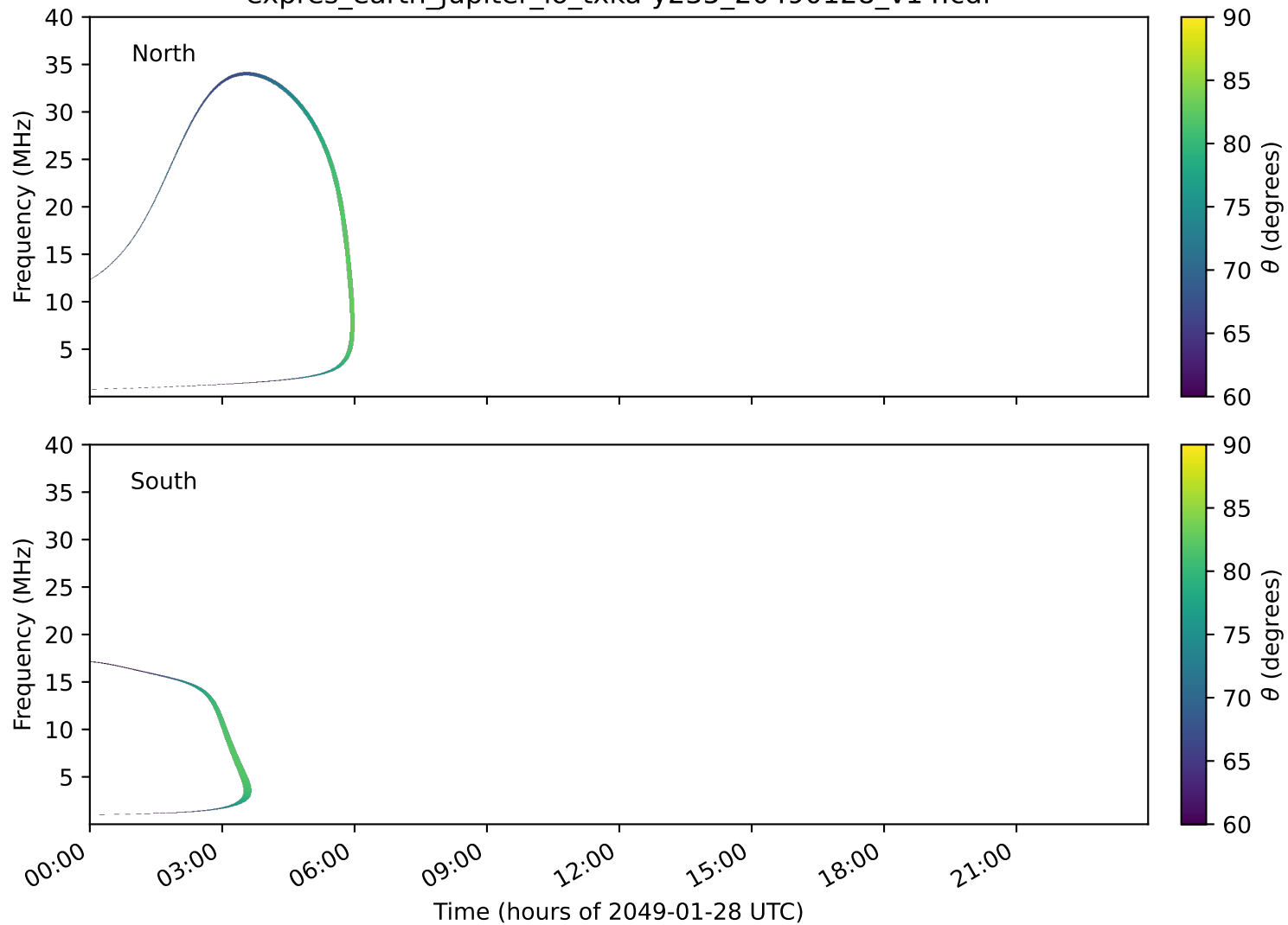
expres_earth_jupiter_io_txka-y235_20490128_v14.cdf
