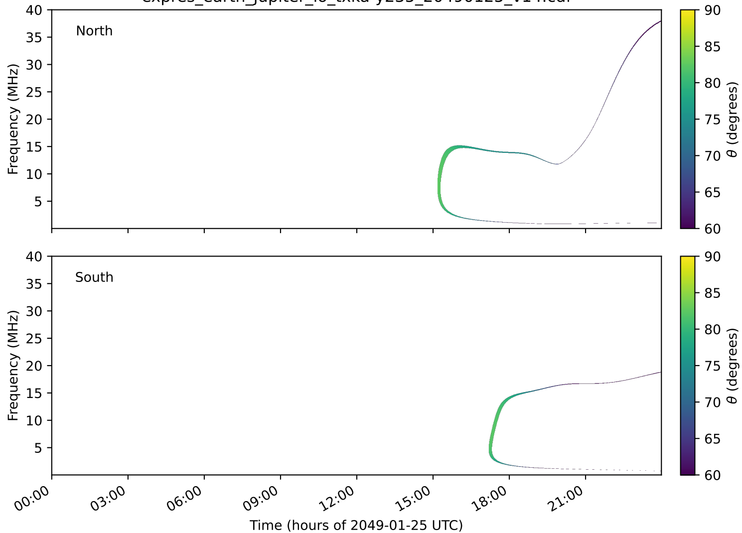
expres_earth_jupiter_io_txka-y235_20490125_v14.cdf
