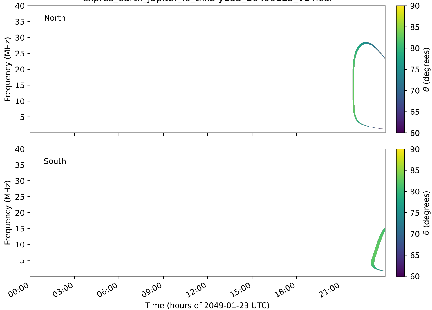
expres_earth_jupiter_io_txka-y235_20490123_v14.cdf
