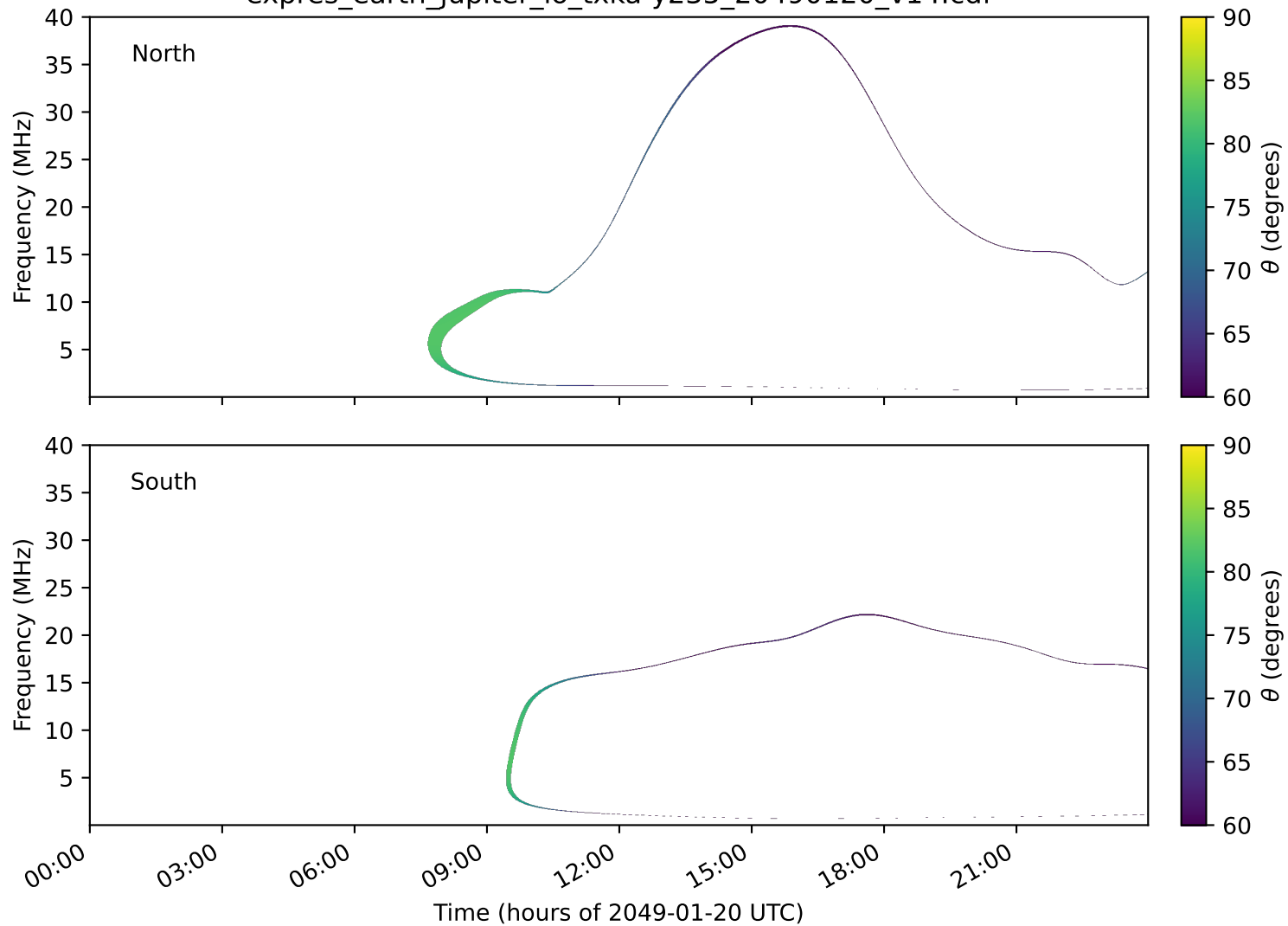
expres_earth_jupiter_io_txka-y235_20490120_v14.cdf
