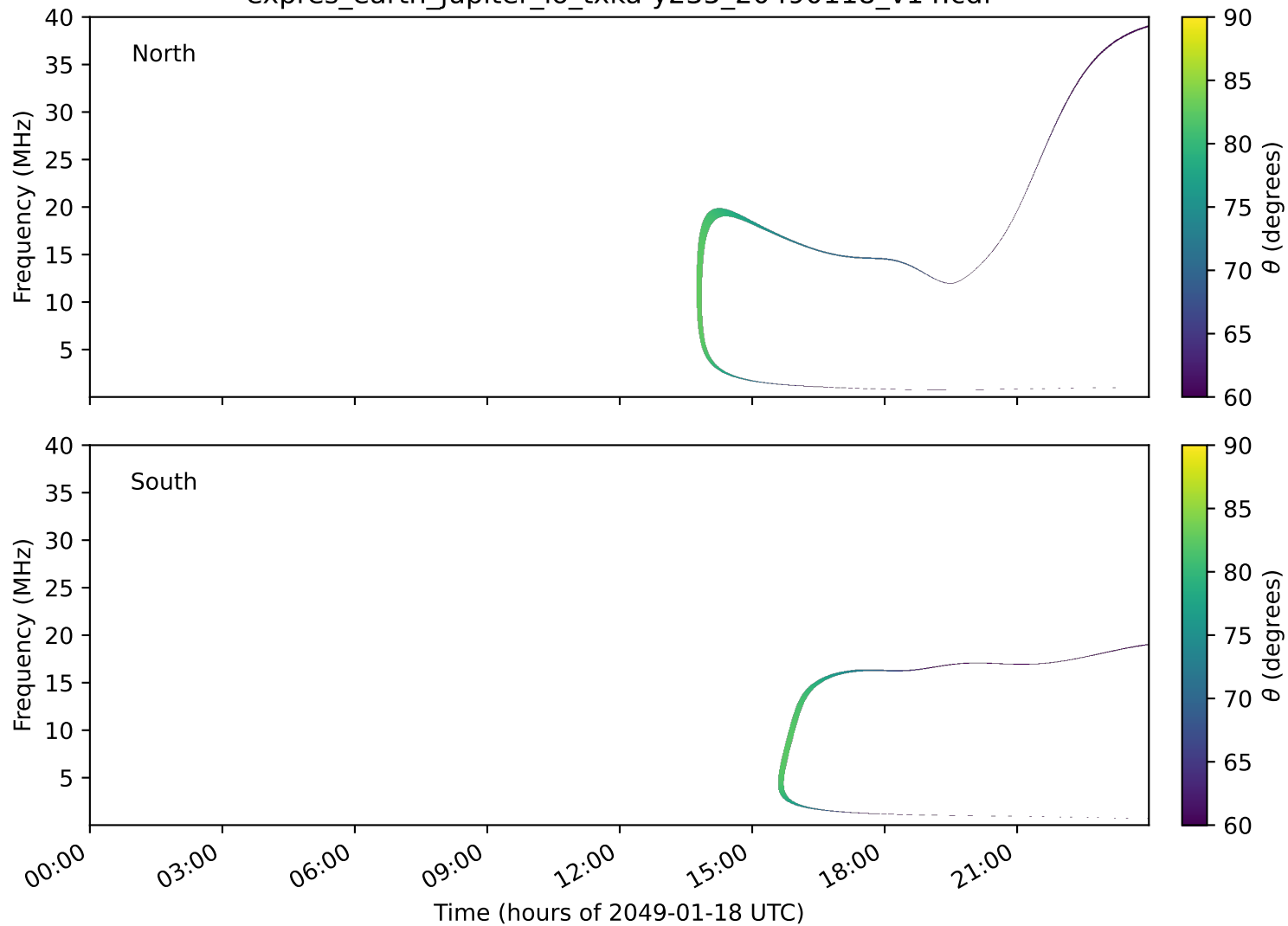
expres_earth_jupiter_io_txka-y235_20490118_v14.cdf
