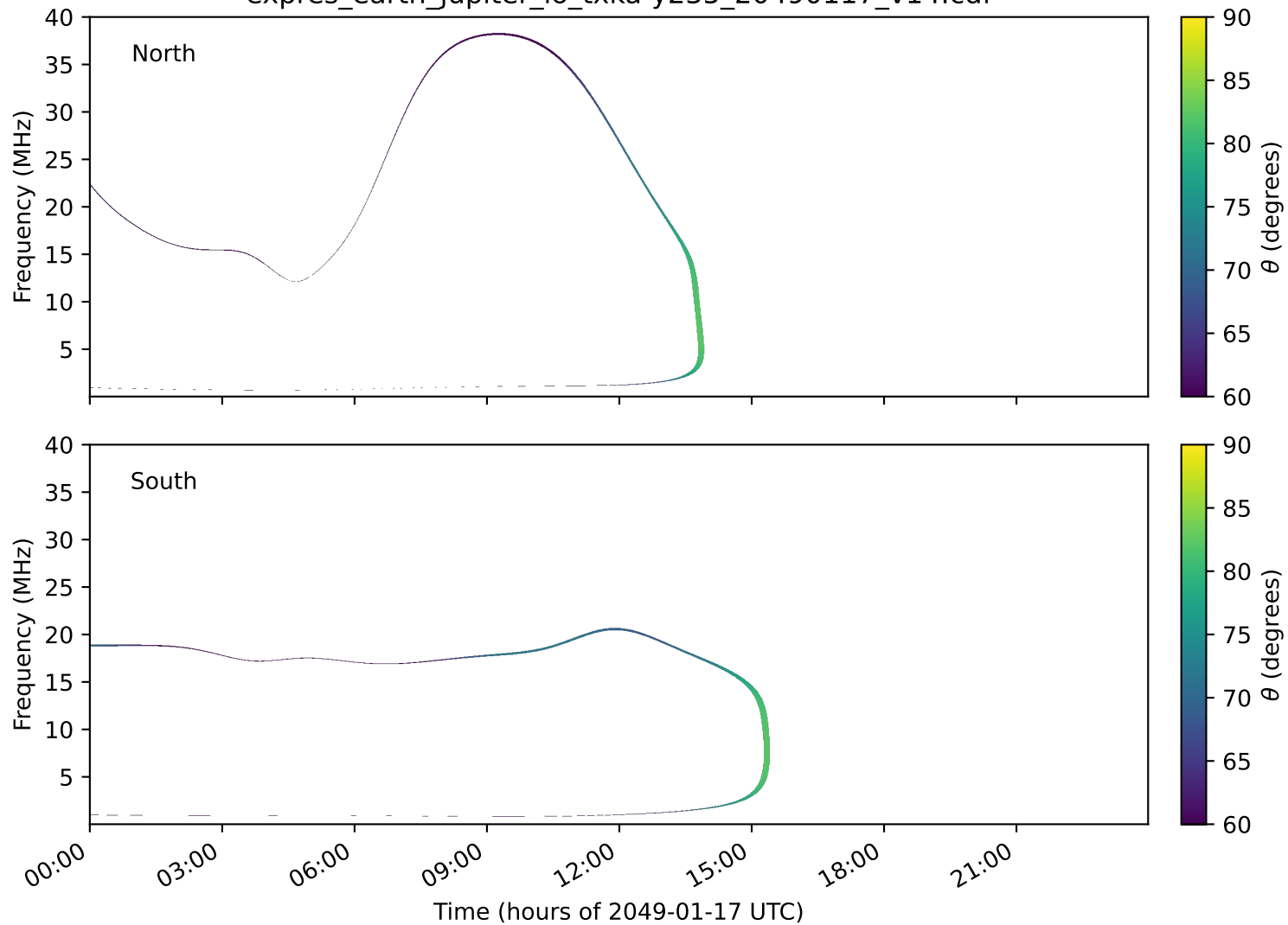
expres_earth_jupiter_io_txka-y235_20490117_v14.cdf
